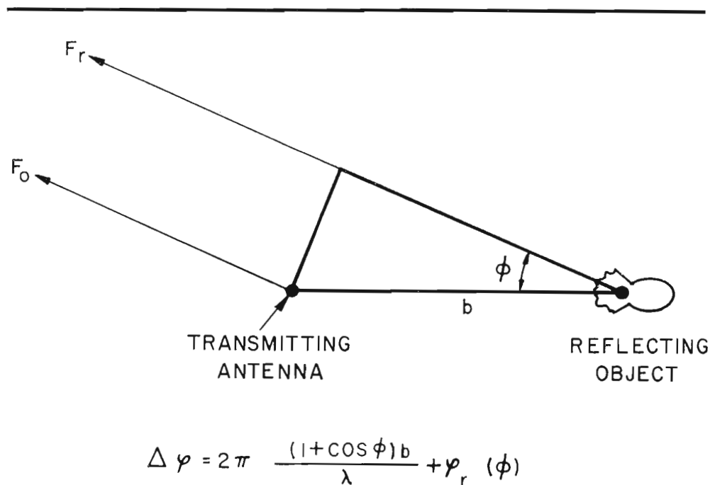
FIG. 1. Geometry which determines horizontal pattern distortion.
