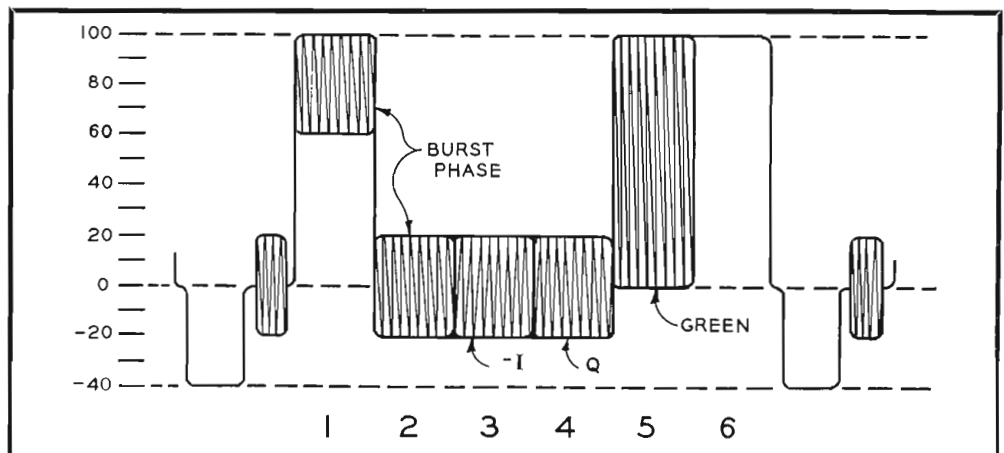
FIG. 1. Waveform sketch of a six-interval reference signal developed and tested by RCA and NBC. For convenience, this will be designated the "Mark I" proposal.
