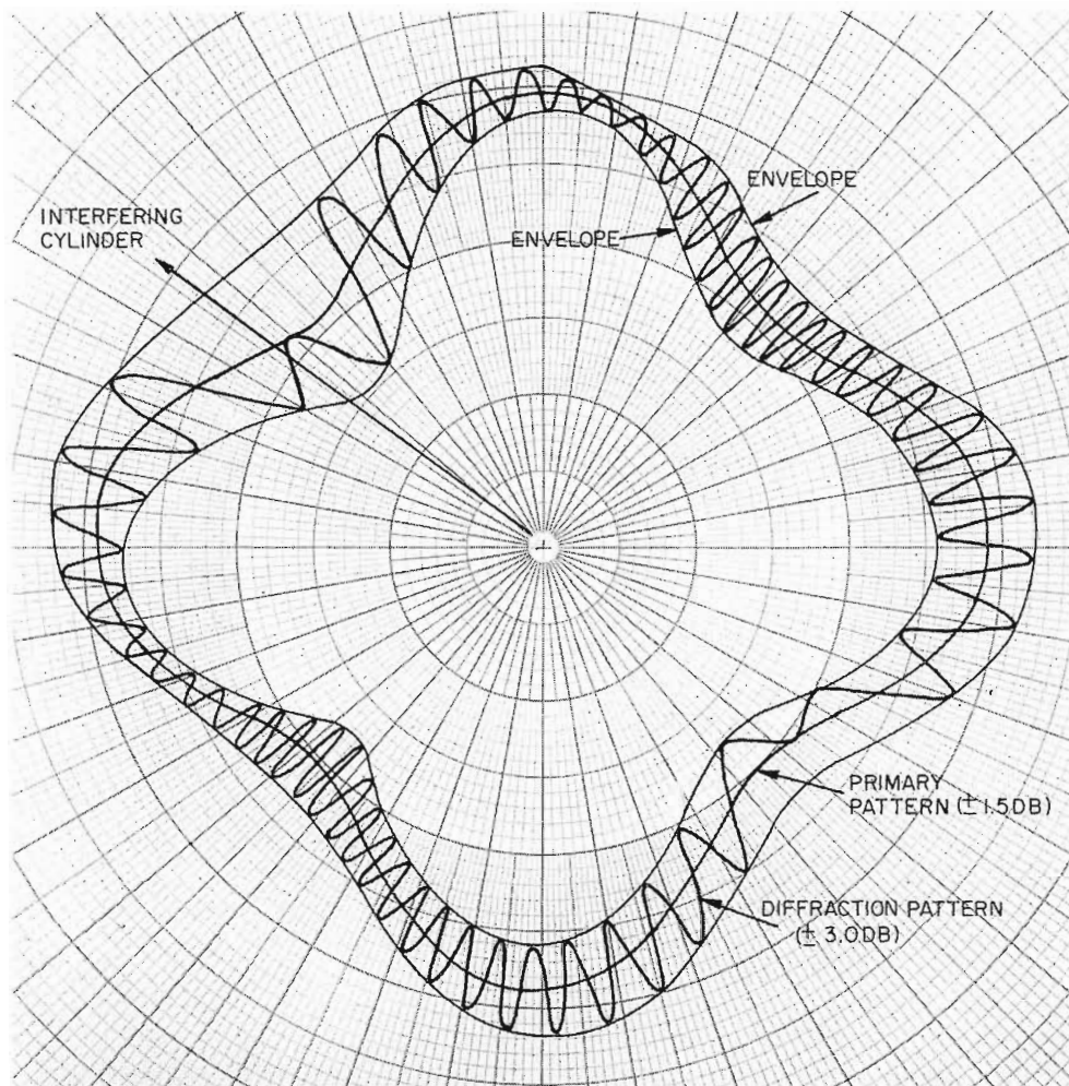
FIG. 2. Calculated horizontal pattern of a Superturnstile antenna in presence of a long vertical highly conducting cylinder of 1.3\lambda diameter about 15\lambda away.
