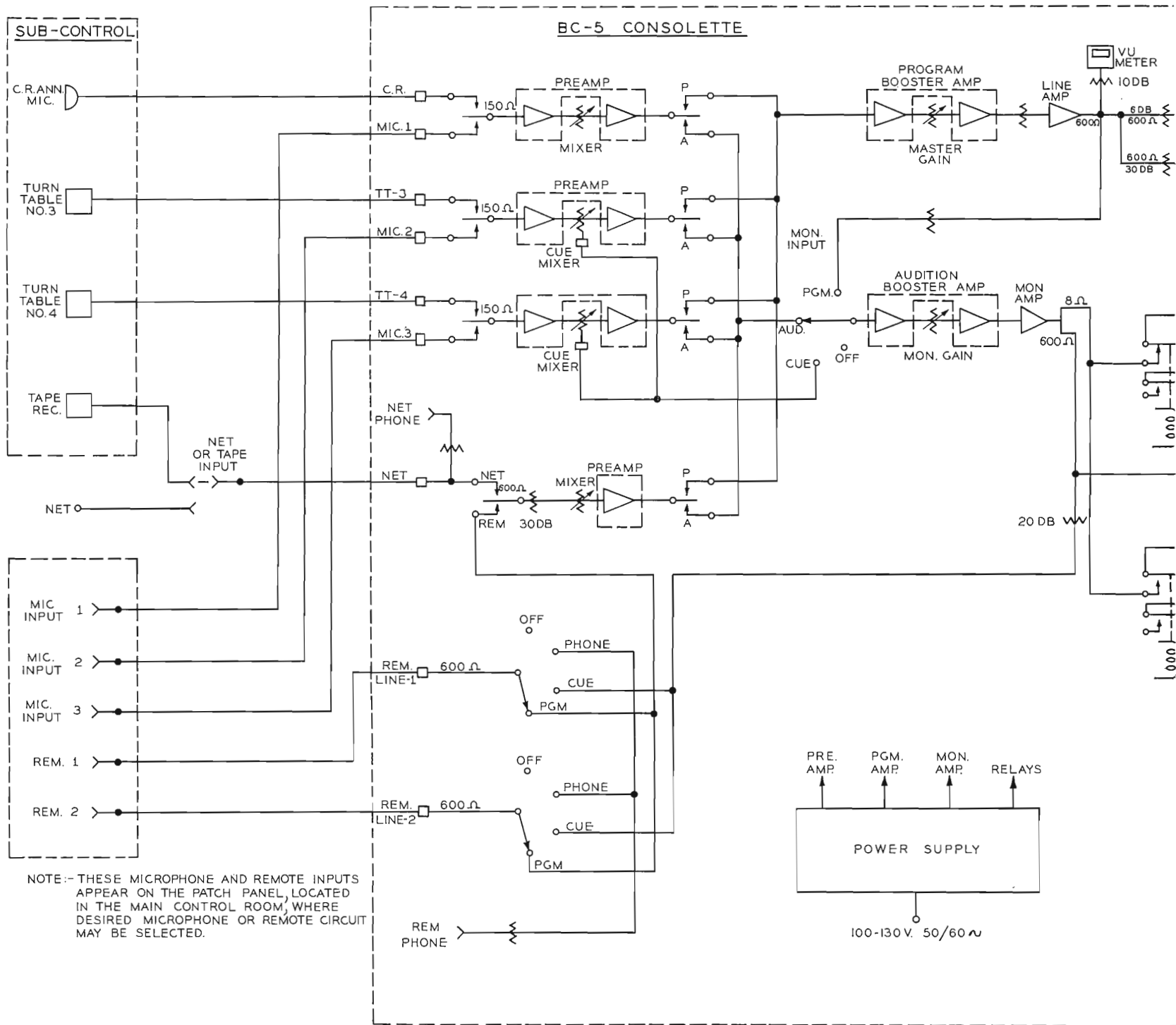
FIG. 14. Subcontrol Block Diagram for Plan C, using the BC-5 Console.
