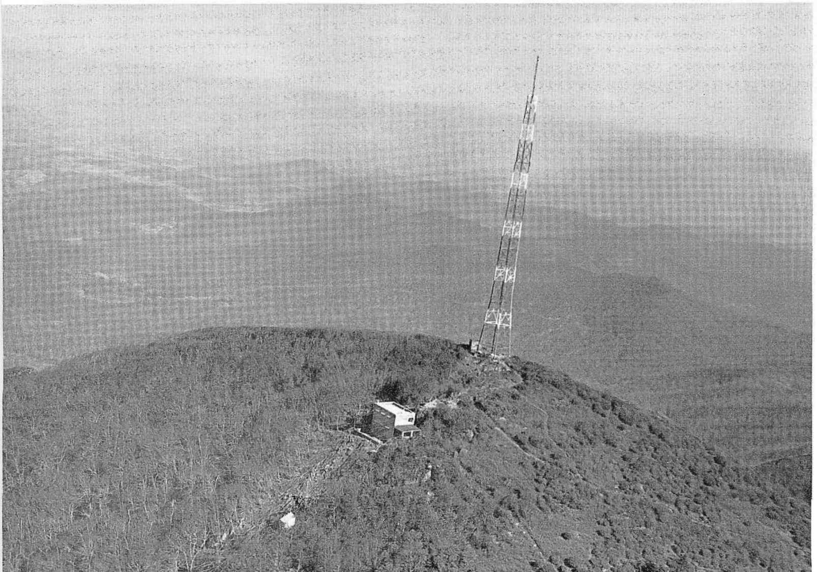
FIG. 1. Aerial view of the WLOS-TV transmitter site atop Mt. Pisgah shows rugged terrain. Transmitter building is structure located in the foreground. Studios are located off to the left about 18 airline miles away in residential area of Asheville, N. C.
