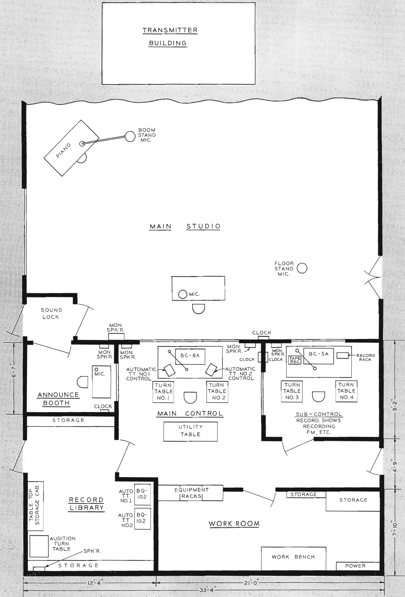
FIG. 12. This shows location of all major equipment items. It is a very complete arrangement embodying a large studio which may be expanded as desired. Note that the transmitter is separated from the studio location.
