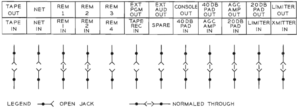
FIG. 2. Jack panel for Plan A.
