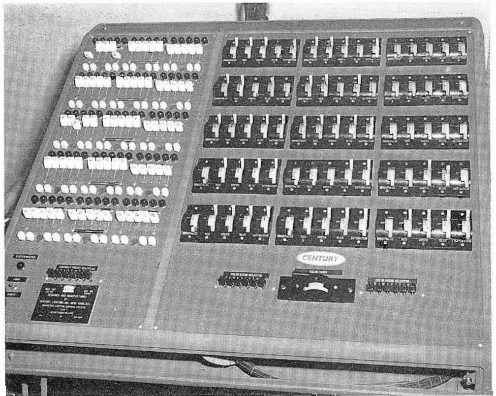
FIG. 6. Five-scene preset control panel for C-lectrochrome magnetic amplifier four-color selective color control system.
