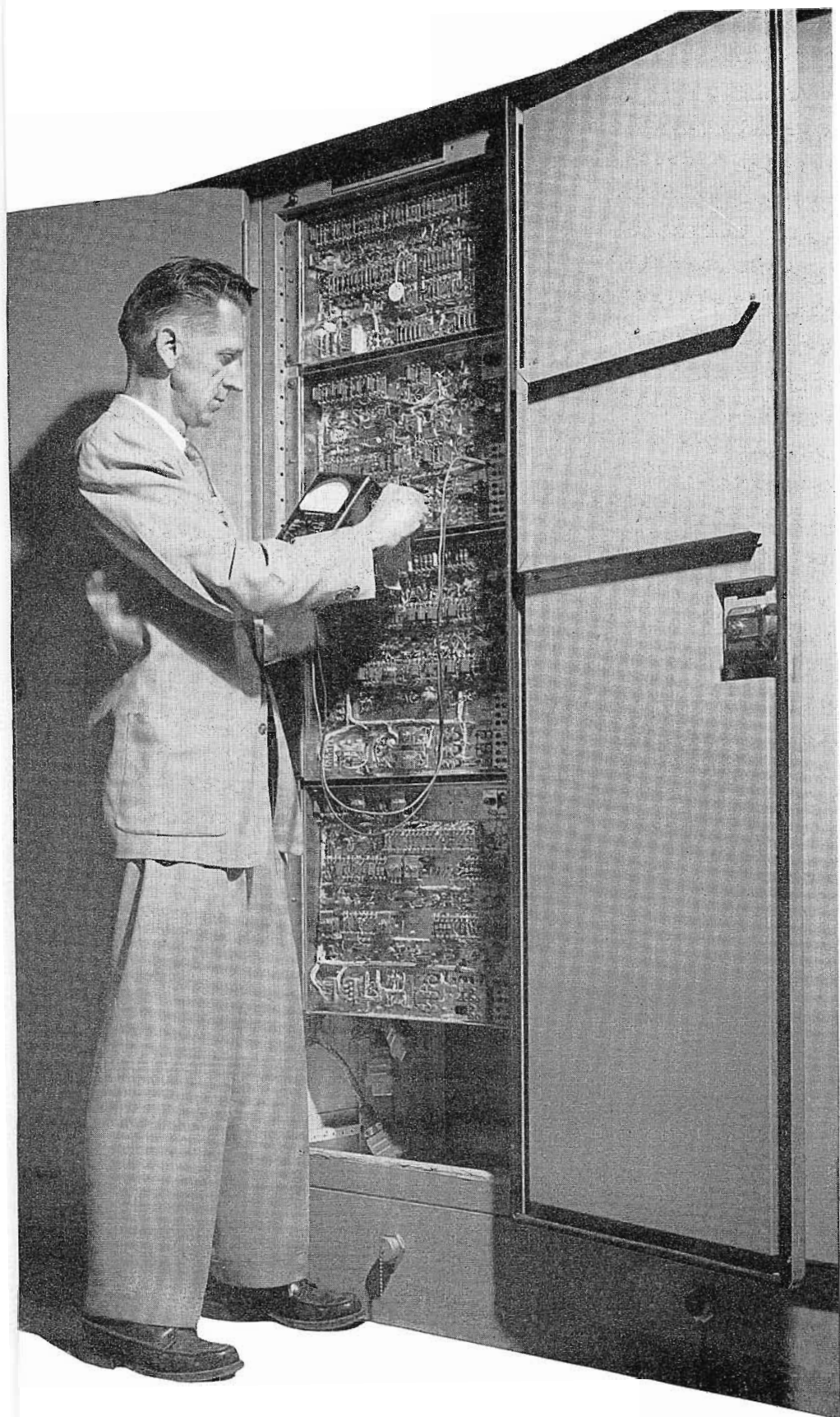
FIG. 4. Merritt Sheeder, Project Engineer, is making a circuit check at the readily accessible underside of an Instrumentation Radar Chassis.
