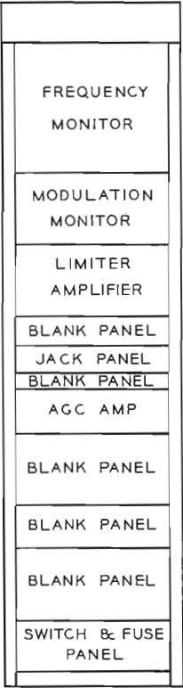
FIG. 3. Rack layout for Plan A equipments. Note blank panels which allow for future expansion.
