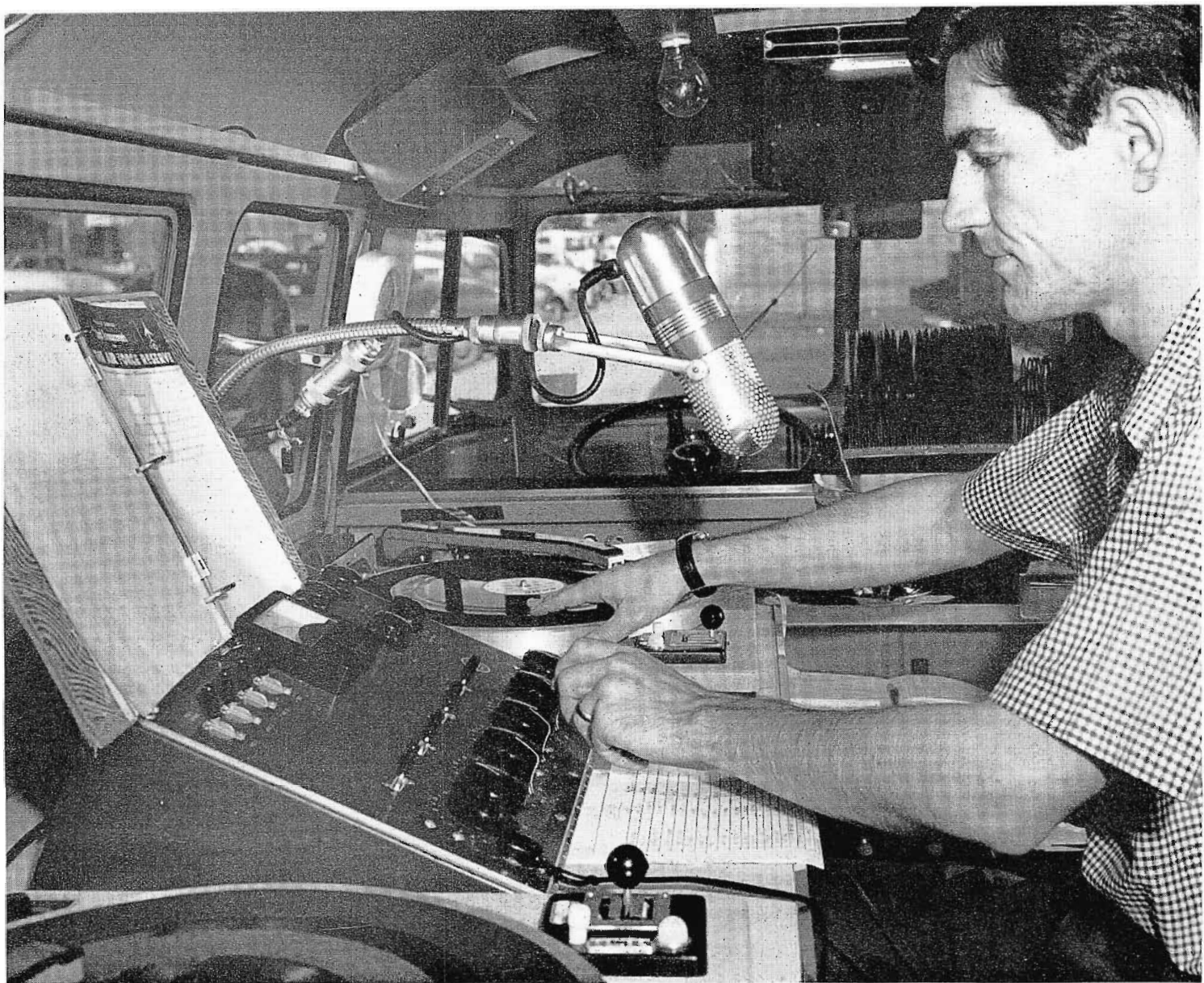
FIG. 3. Complete D-J studio is built into KRMG mobile unit using Type BC-5A Audio Consolette. There is sufficient room for convenient operation.
